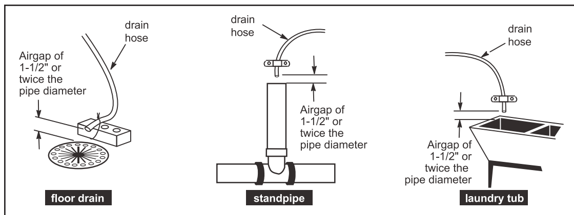
Typical Drain Line Installations
